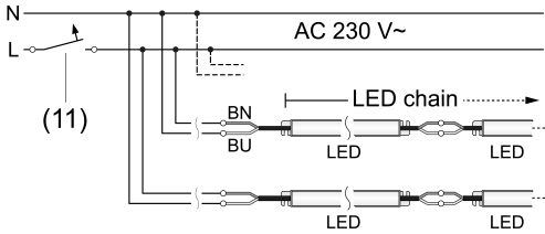
Figure 6: Circuit diagram
