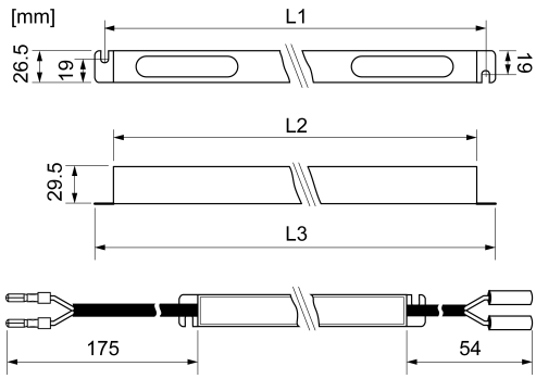
Figure 4: Dimensioned drawing
