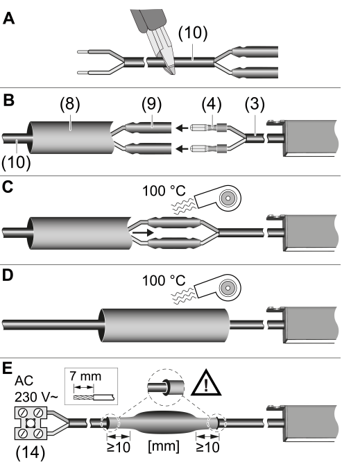
Figure 9: Connecting the first light insert to the supply line (Standard luminaire + adapter cable)
