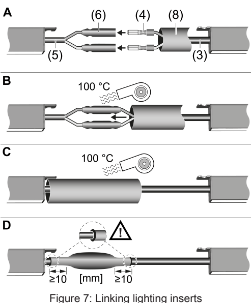
Figure 7: Linking lighting inserts
