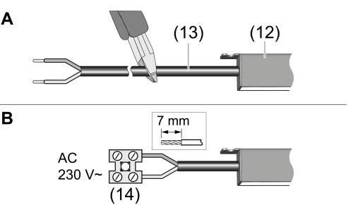
Figure 10: Connecting the first light insert to the supply line (special luminaire with long input cable)
