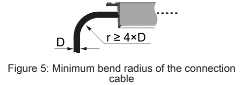
Figure 5: Minimum bend radius of the connection cable
