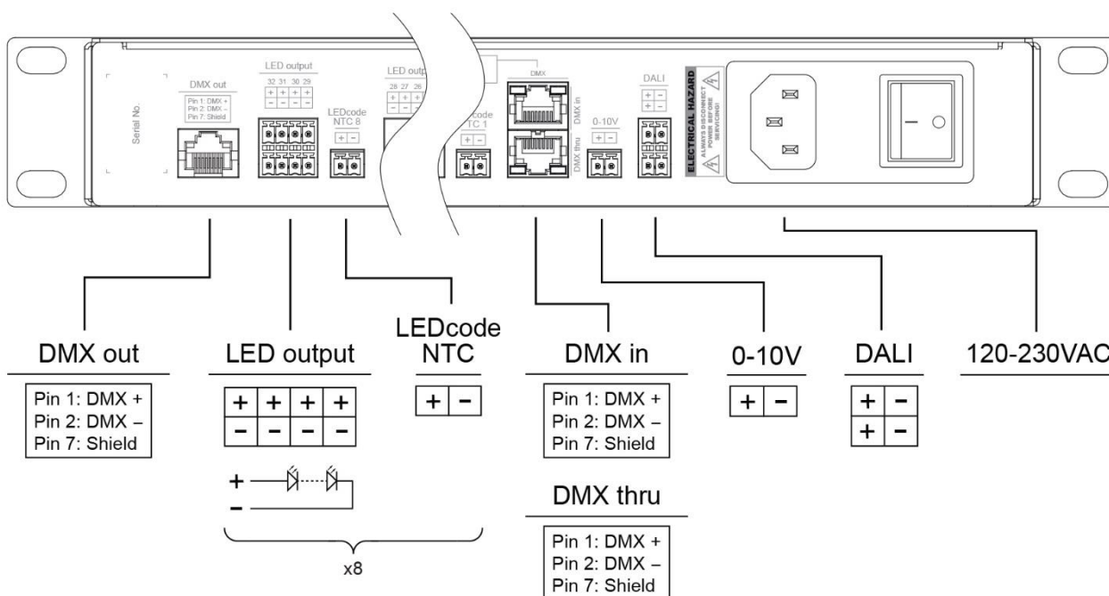
Figure 2.1 POWERdrive 6060/R connections
