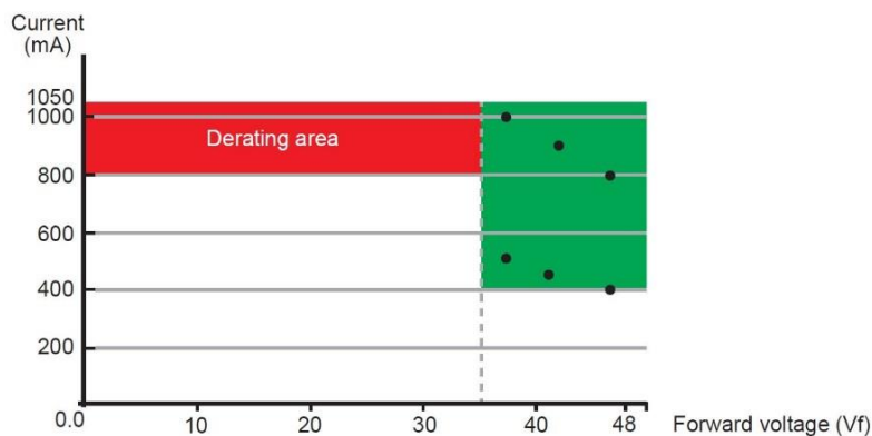
Figure 1.1 Derating diagram
