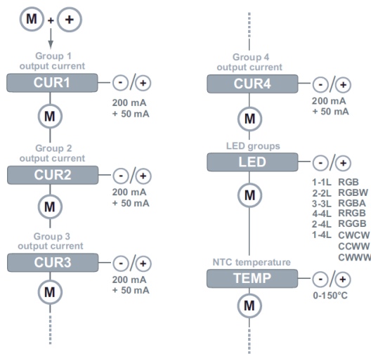
Figure 4.2 Configuring LED output current, LED group configuration, NTC temperature
