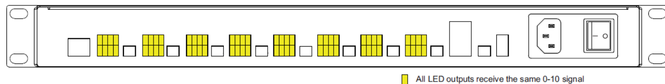
Figure 2.6 One 0-10V control channel
