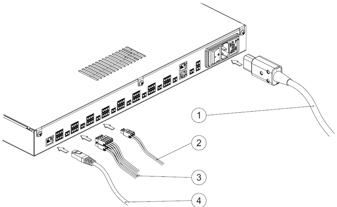
Figure 3.1 Cable connections: mains cable (1), NTC and LEDcode wires (2), LED wires (3) and DMX cable (4)
