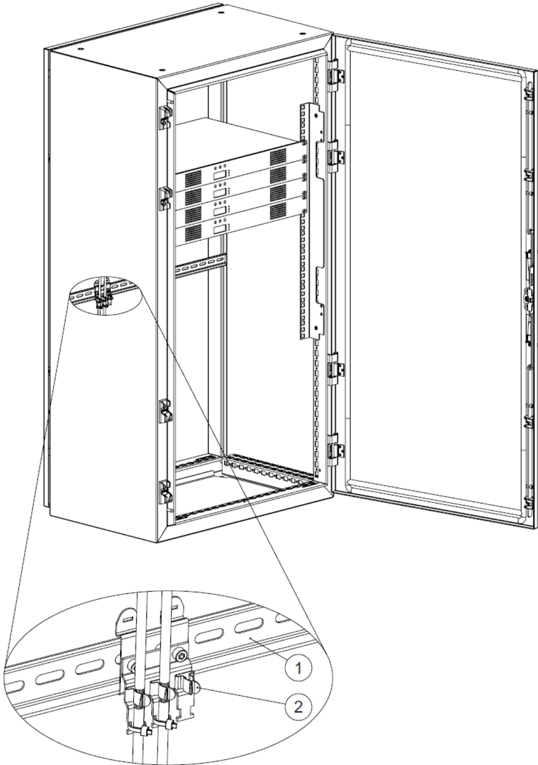
Figure 3.2 Grounding LED wires inside 19" rack unit
