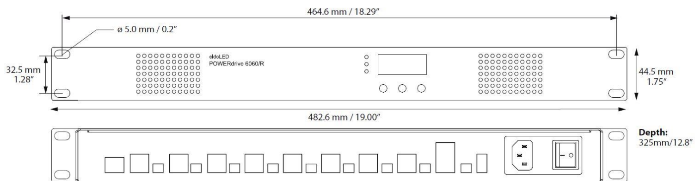
Figure 1.2 POWERdrive 6060/R dimensions
