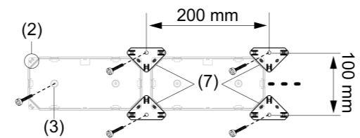
Figure 6: Mounting with connectors LED lamp PR100
