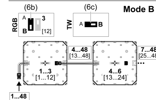
Figure 11: Setting operating mode for addressing
