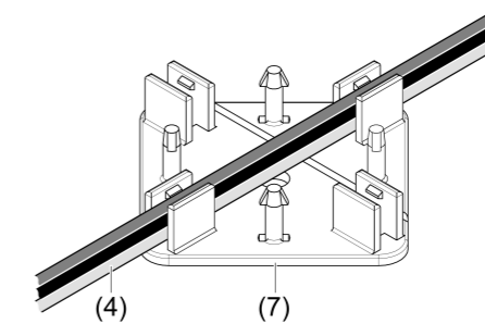
Figure 9: Laying the supply line
