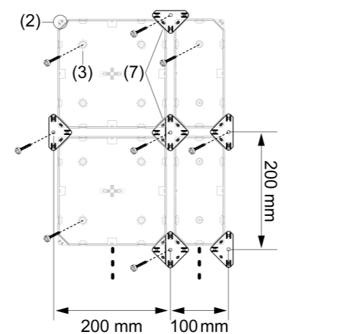
Figure 7: Mounting with connectors LED lamp PQ200 and PR100 combined
