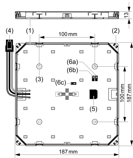
Figure 1: LED lamp PQ200
