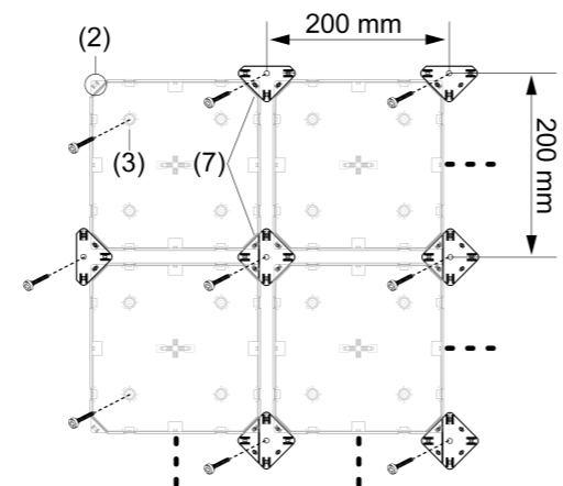
Figure 5: Mounting with connectors LED lamp PQ200
