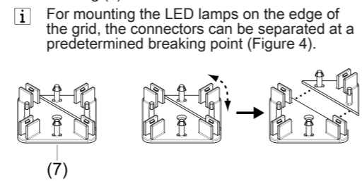
Figure 4: Separating connectors
