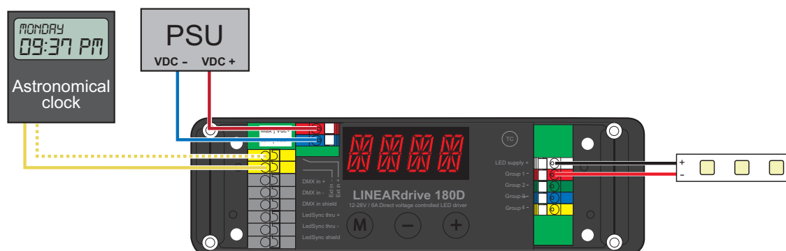
Connecting astronomical clock to LED driver
